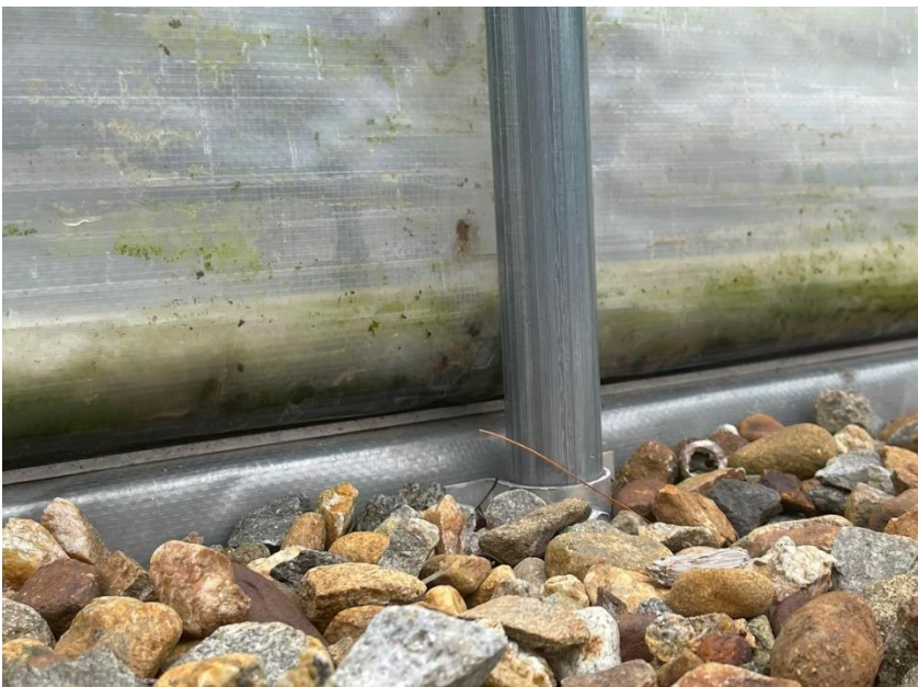
Figure 7. Closeup of seated fabric rail showing adequate but less than complete seal.
